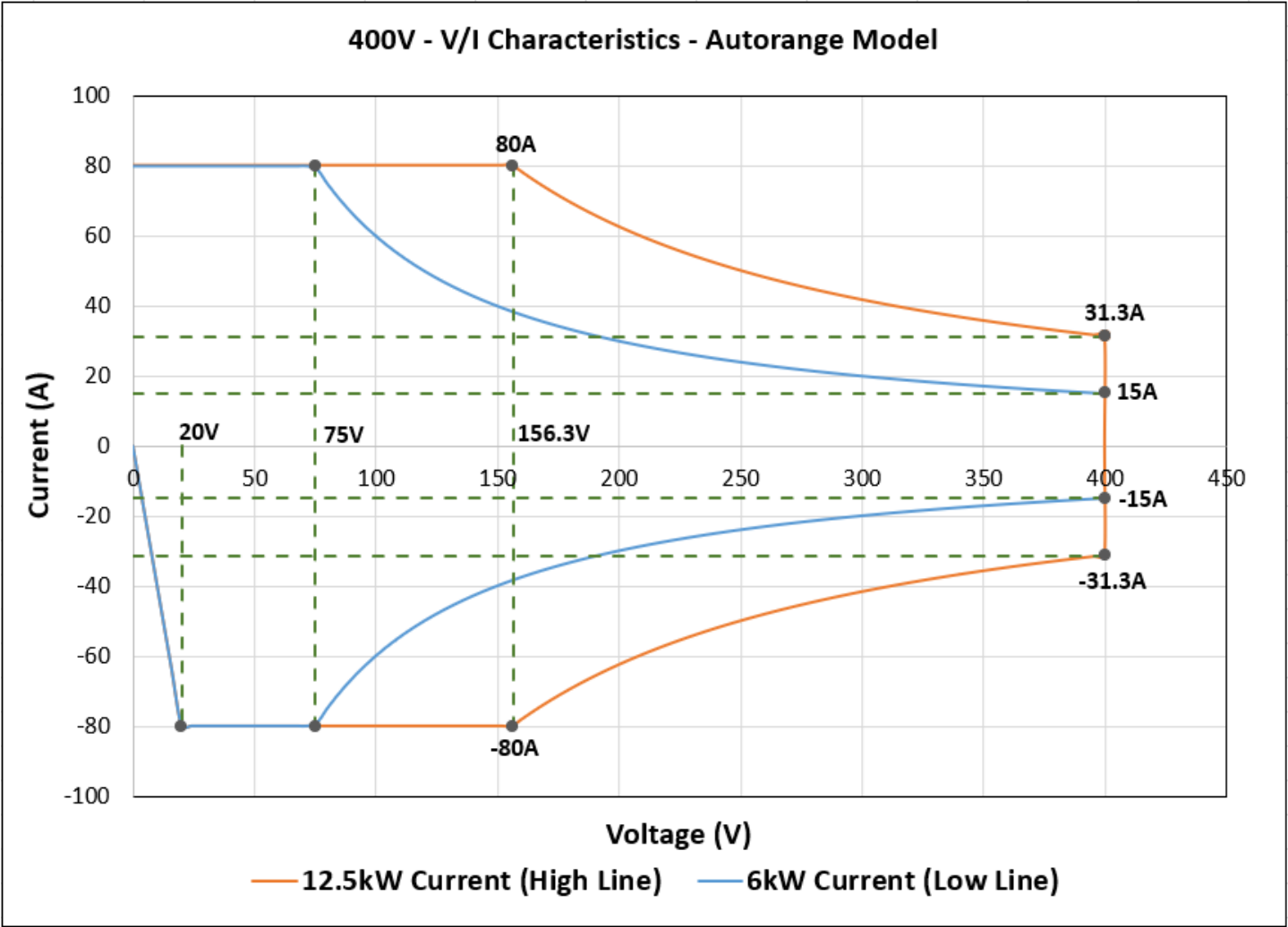
400V 12.5kW 80A model
