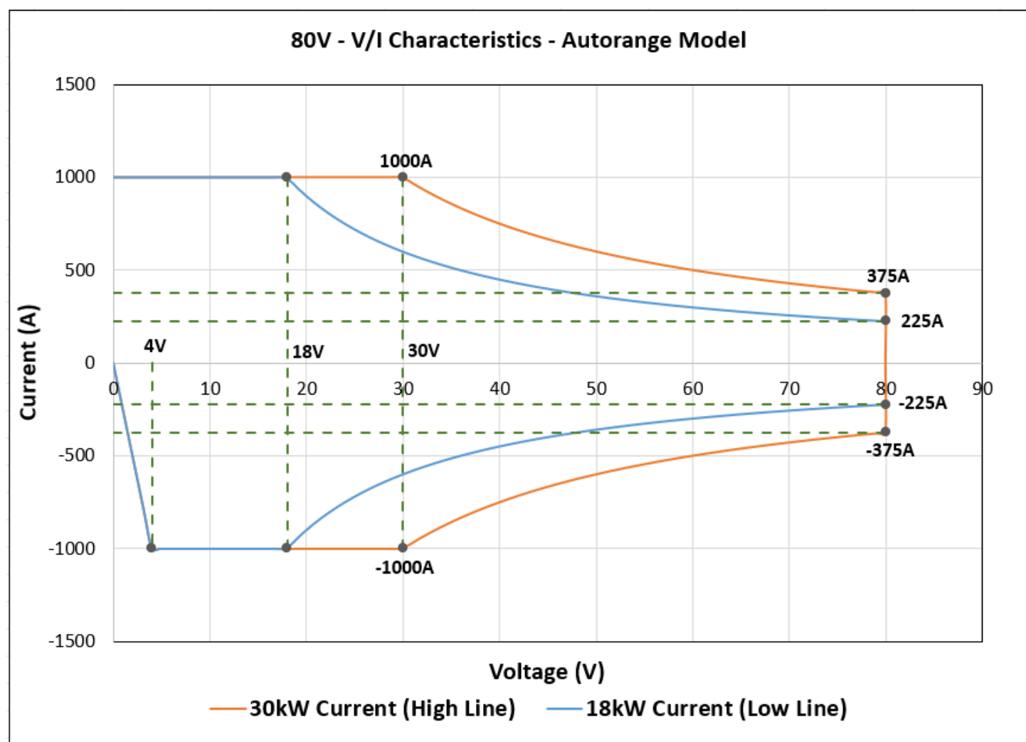
80V 30kW 1000A model
