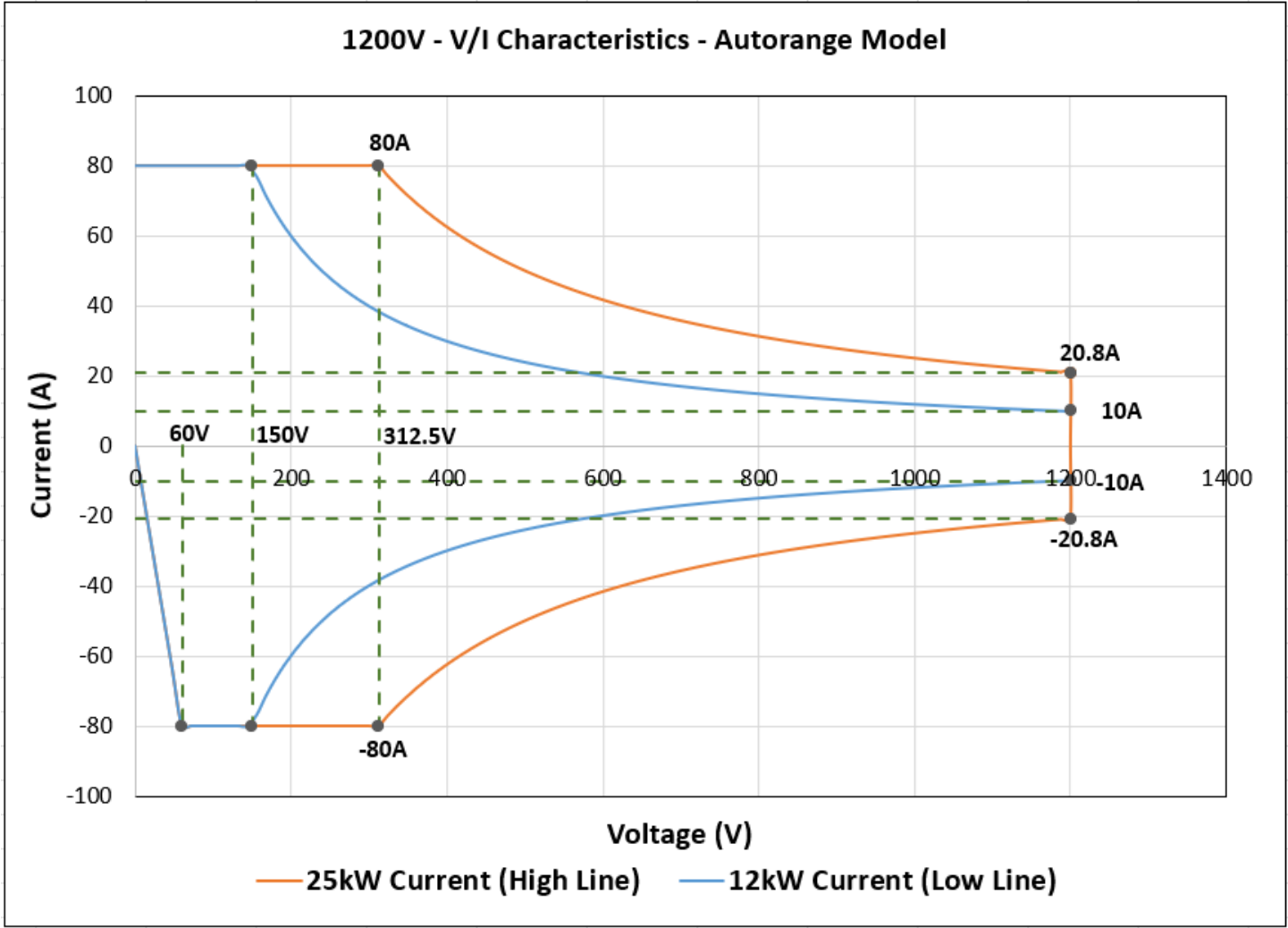
1200V 25kW 80A model
