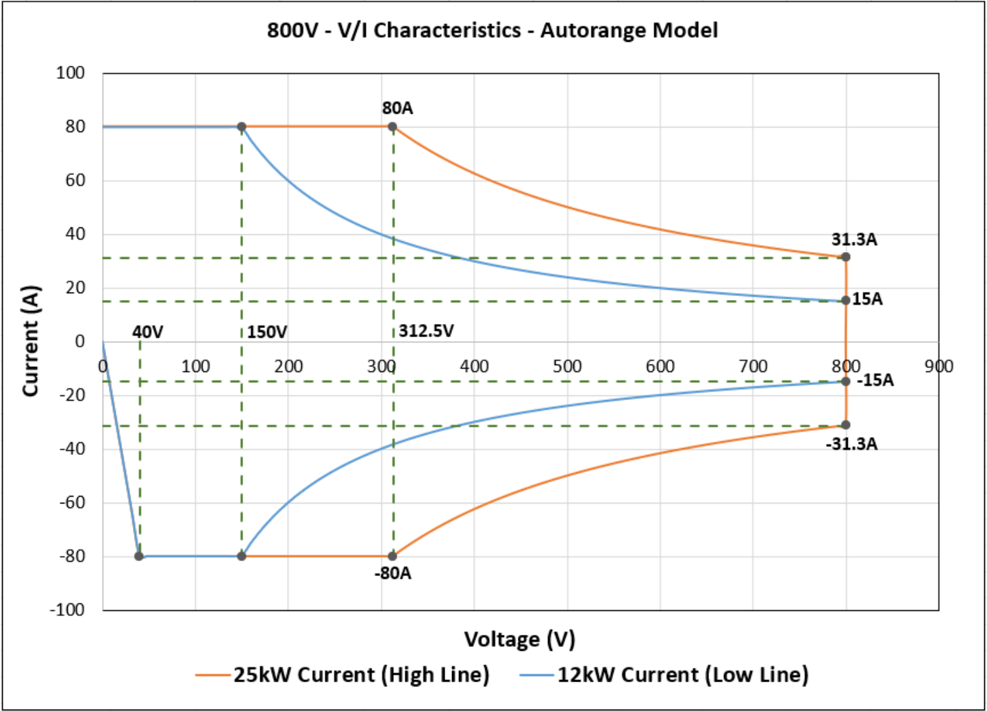
800V 25kW 80A model
