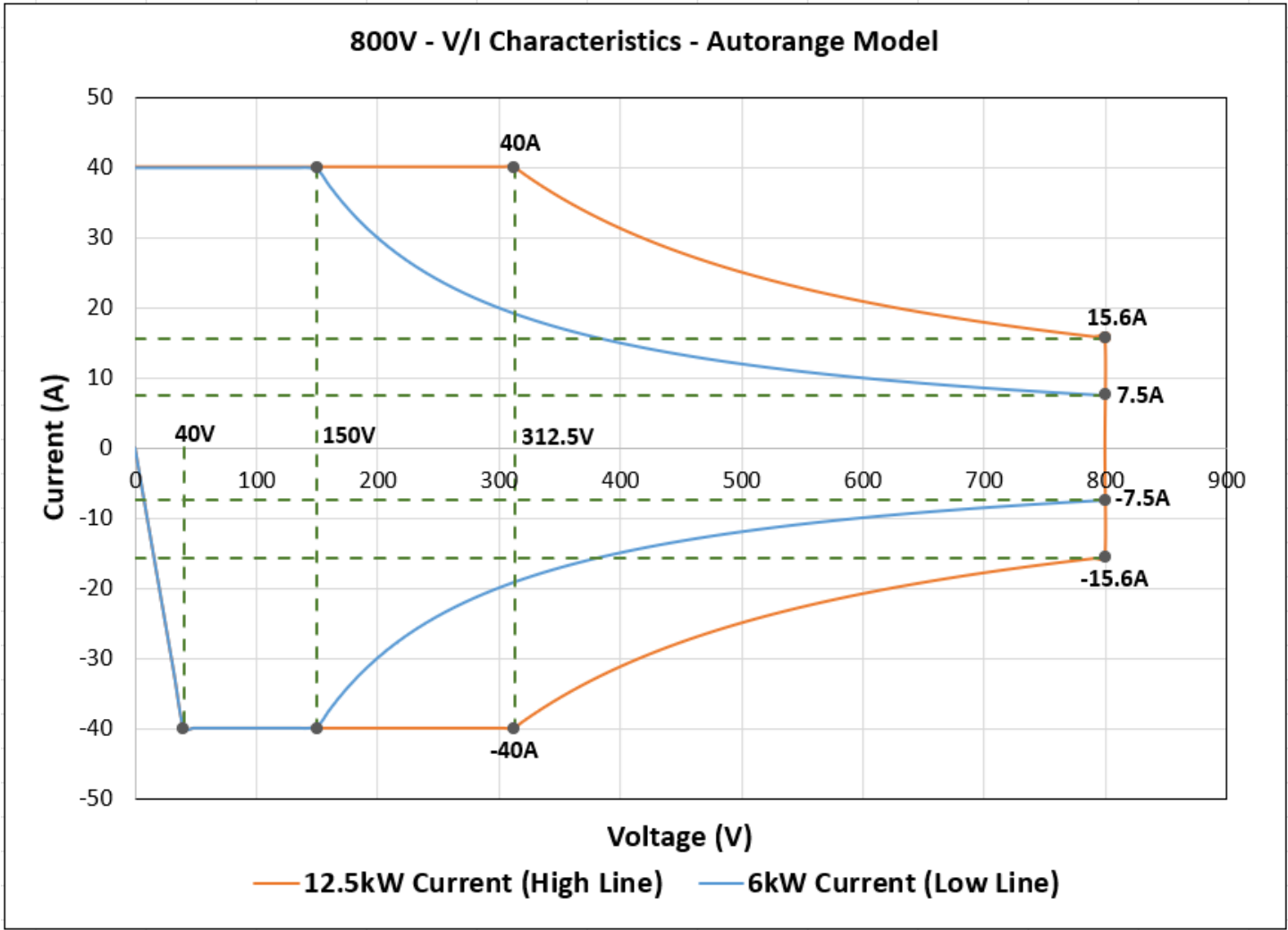
800V 12.5kW 40A model
